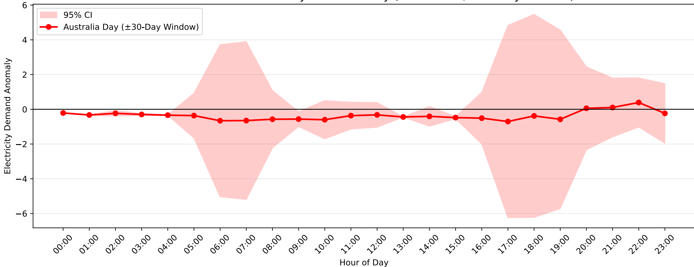
Harbord Demand Anomaly: Australia Day (2004-2005, \pm 30 -Day Window)
